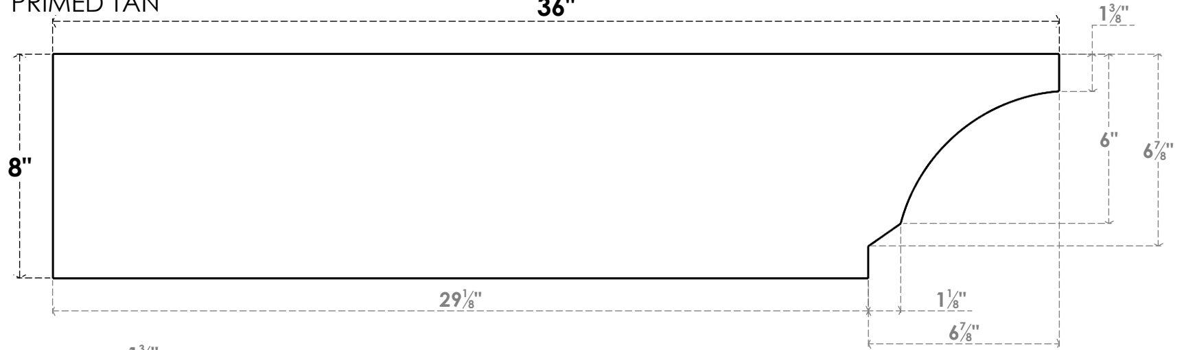
SIDE PROFILE
